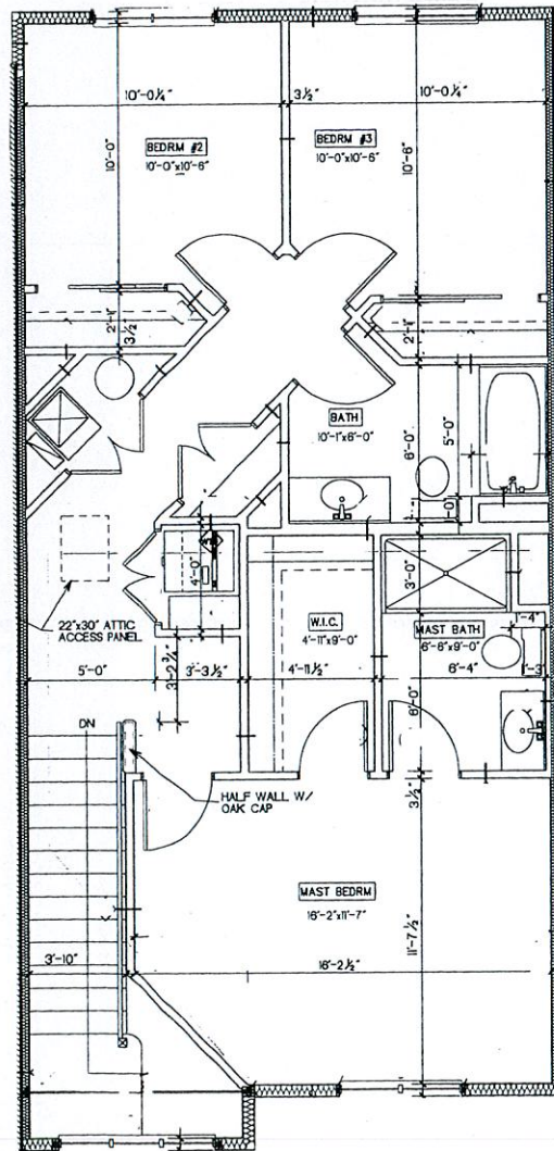
2ND FLOOR
