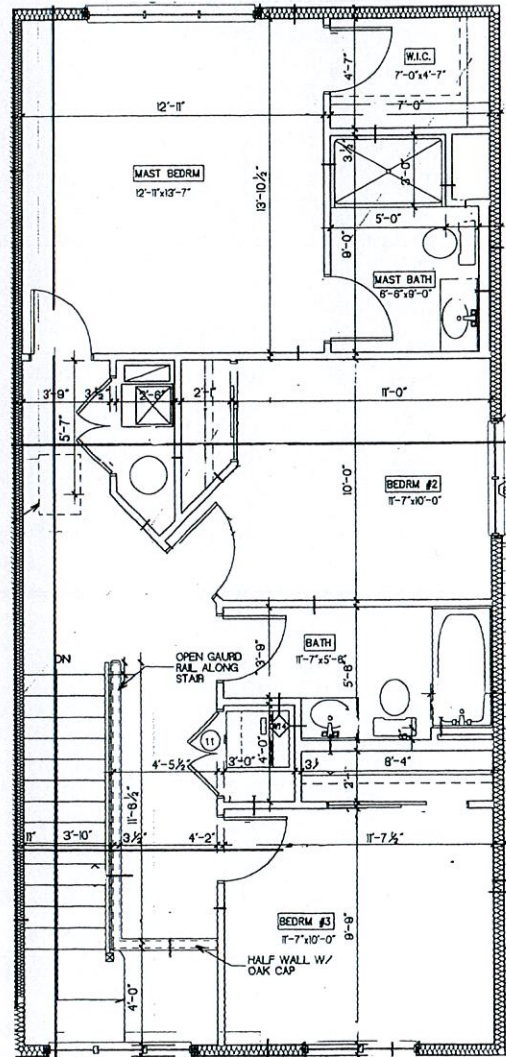
2ND FLOOR
